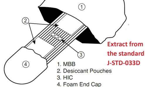
Figure 3-1 Typical Dry-Pack Configuration for Moisture-Sensitive SMD Packages in Shipping Tubes
